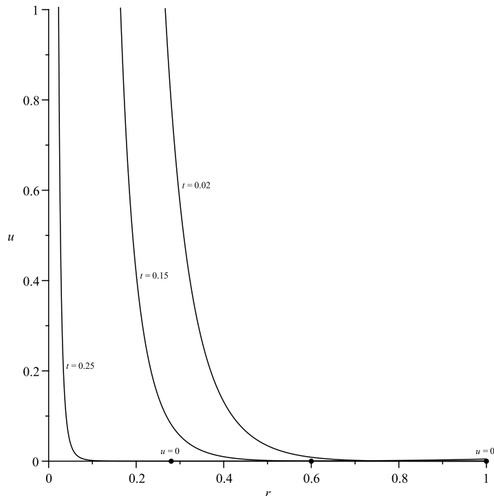
FIGURE 2. Graph of solution (78) with n = 6 ( q + 1 = 1/2 ).
