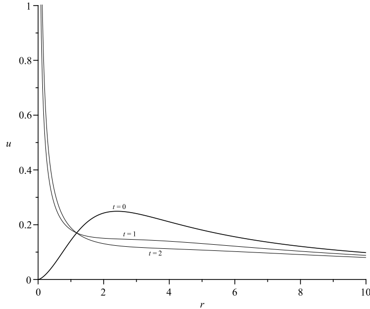
FIGURE 4. Graph of solution (65).
