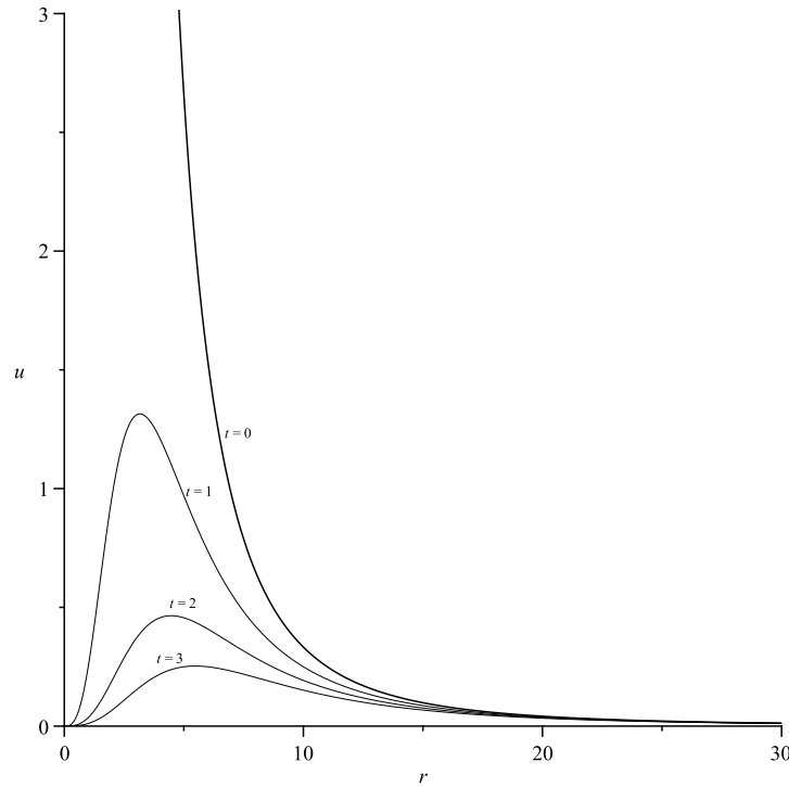
FIGURE 3. Graph of solution (95) with \nu = 3 .
