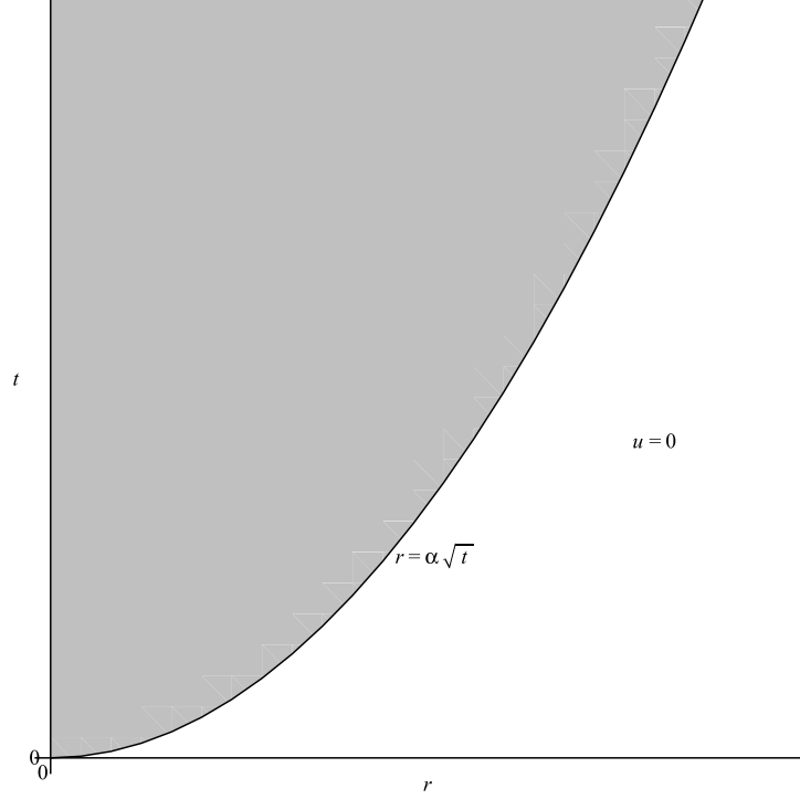
FIGURE 1. Space-time graph for solution (78).
