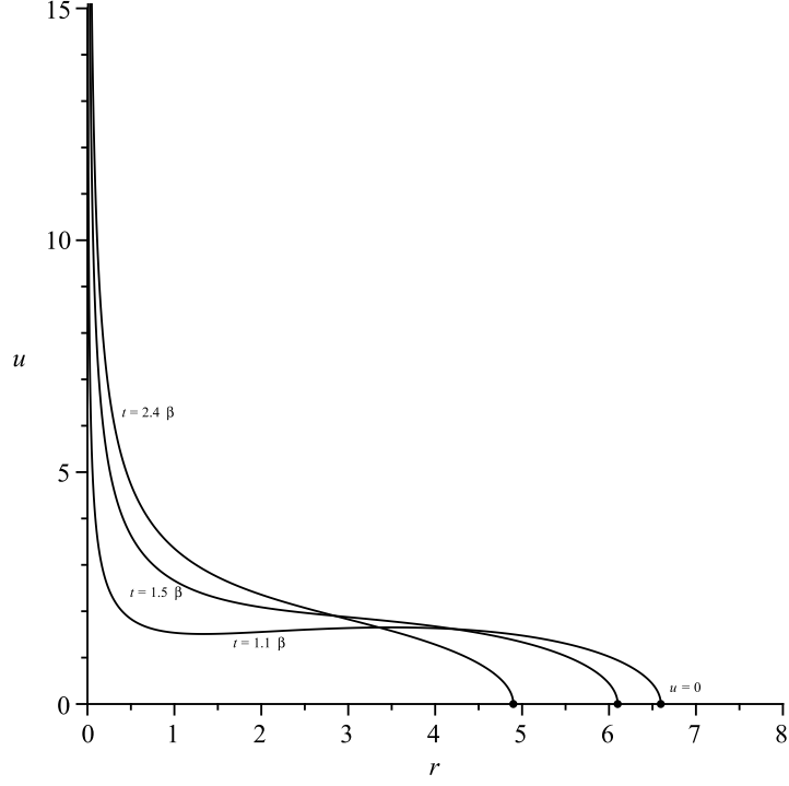
FIGURE 6. Graph of solution (100) with \beta = 5 , \alpha = 20 .
