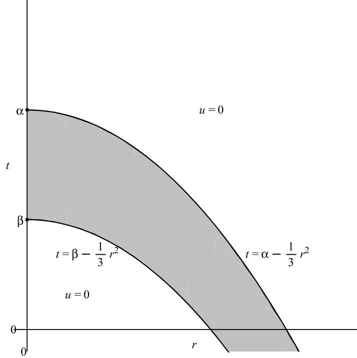
FIGURE 5. Space-time graph of solution (100).
