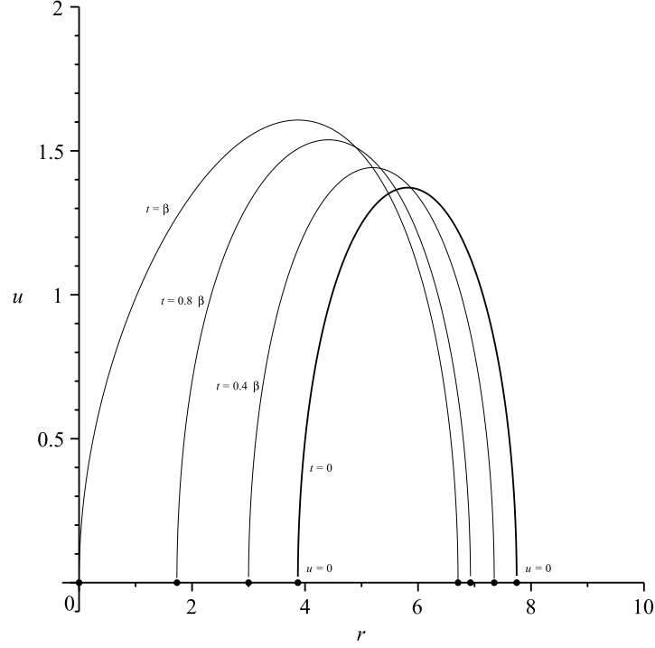
FIGURE 7. Graph of solution (100) with \beta = 5 .
